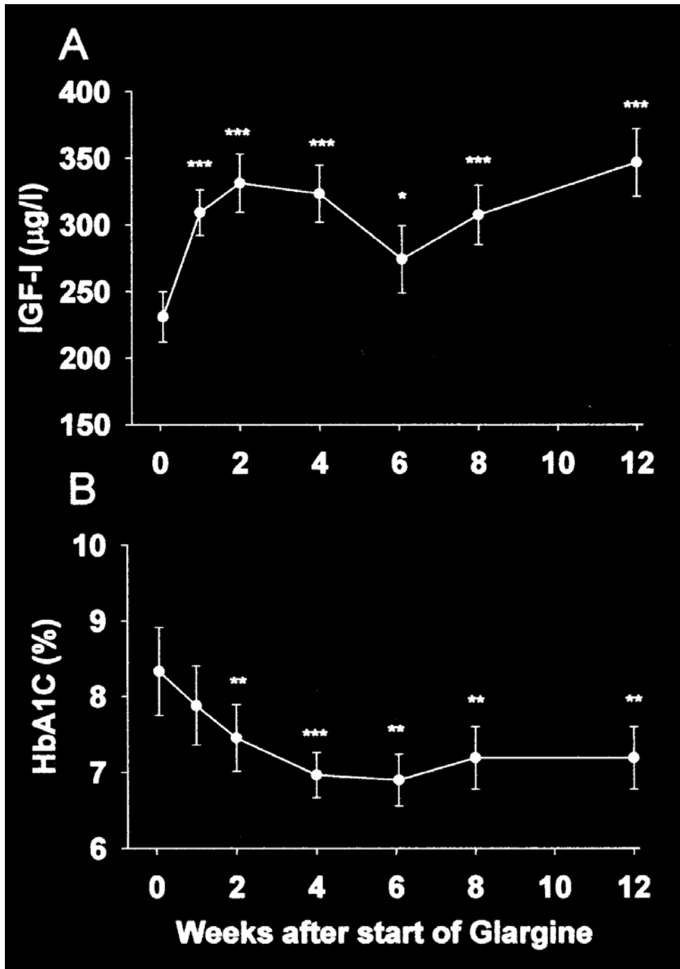
Figure 1: IGF-I (A) and HbA1c (B) on meal insulin therapy using basal NPH insulin (MIT/NPH) at basal (0 weeks) and during 12 weeks on MIT/Glargine treatment in 12 adolescents with T1DM. * P < 0.05 , ** P < 0.01 , *** P < 0.001
