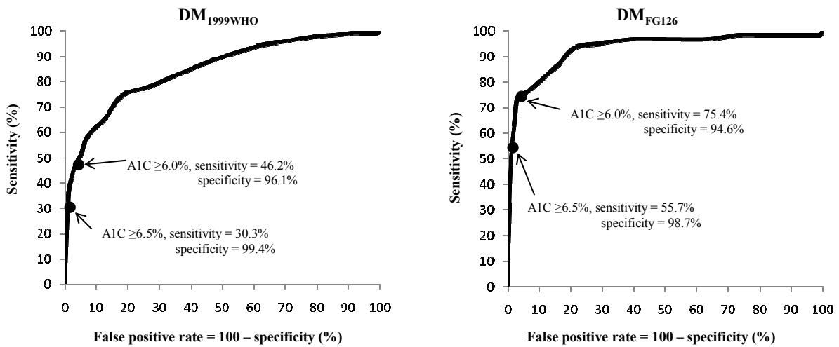
Figure. ROC curves of hemoglobin A1c for detecting subjects with DM_{1999WHO} and DM_{FPG126}
