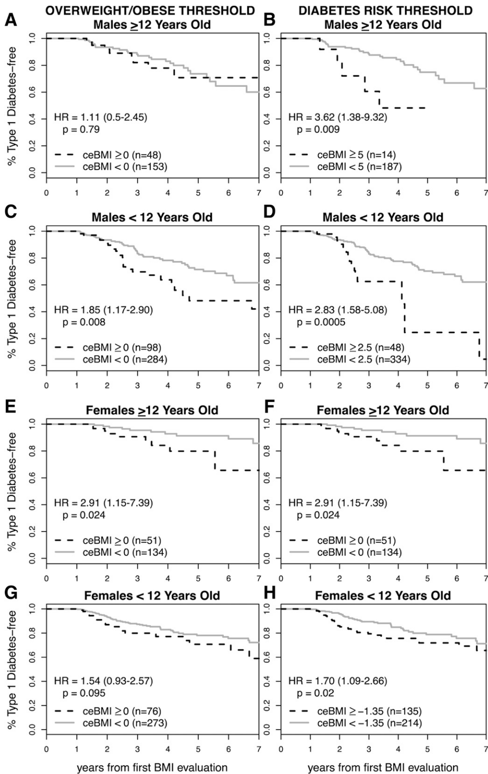
Figure 1 —Effect of ceBMI on type 1 diabetes risk comparing traditional overweight/obese ceBMI definitions to age- and sex-specific ceBMI diabetes risk thresholds. Proportion type 1 diabetes free among pediatric subjects of the PTP cohort for age ( \geq 12 vs. < 12 years old) and sex strata (males vs. females). A, C, E, and G: Assessment of overweight/obese threshold based on 85th percentile for age- and sex-adjusted BMI. Dotted lines indicate ceBMI \geq 0 (overweight/obese); solid gray indicates ceBMI < 0 (nonoverweight/obese). B, D, F, and H: Assessment of ceBMI diabetes risk thresholds identified by recursive partitioning. Dotted lines indicate greater than or equal to age- and sex-specific ceBMI diabetes risk threshold; solid gray indicates less than age- and sex-specific ceBMI diabetes risk threshold. All models adjusted for antibody number (single vs. multiple).
